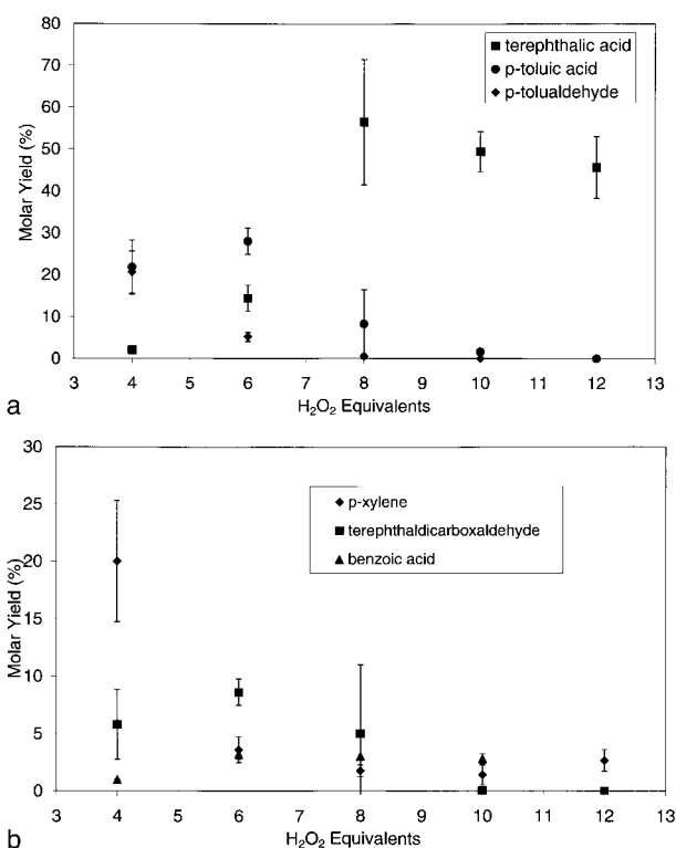
Figure 7. Product molar yields from p -xylene oxidation in SCW at 380 °C at different H 2 O 2 initial concentrations ( [p\text{-xylene}]_0 = 0.08\text{ M} , [\text{MnBr}_2] = 7.7 \times 10^{-3}\text{ M} , [\text{H}_2\text{O}] = 400\text{ kg m}^{-3} , t = 7.5\text{ min} ); (a) major products, (b) minor products.
