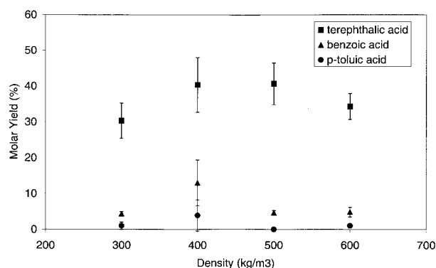
Figure 5. Product molar yields from p -xylene oxidation in SCW at 380 °C at different water densities ( [p\text{-xylene}]_0 = 0.07\text{ M} , [\text{H}_2\text{O}_2]_0 = 0.86\text{ M} , [\text{MnBr}_2] = 7.5 \times 10^{-3}\text{ M} , t = 15\text{ min} ).
