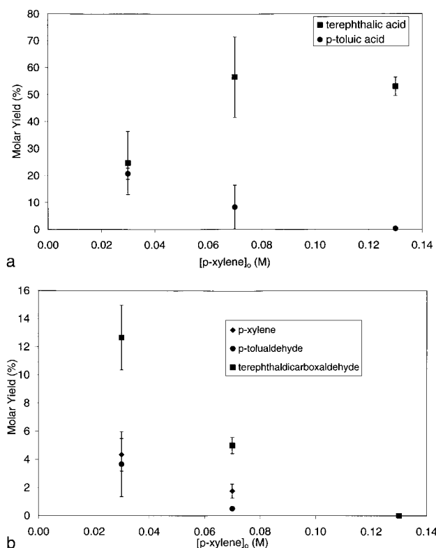
Figure 9. Product molar yields from p -xylene oxidation in SCW at 380 °C at different initial concentrations of p -xylene, H 2 O 2 , and MnBr 2 (H 2 O 2 equivalents = 8, MnBr 2 equivalents = 0.1, [H 2 O] = 400 kg m -3 , t = 7.5 min); (a) major products, (b) minor products.
