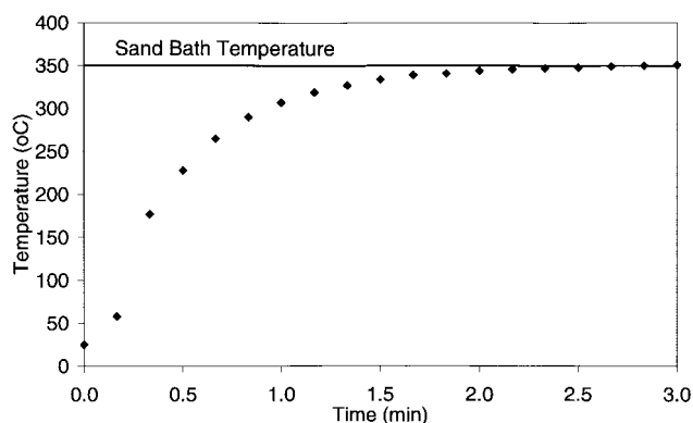
Figure 10. Temperature of a reactor loaded with water versus time in 350^\circ\text{C} sand bath.
