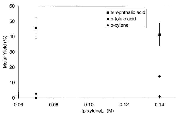
Figure 8. Product yields from p -xylene oxidation in SCW at 380 °C at different p -xylene initial concentrations ([H 2 O 2 ] 0 = 0.8 M, [MnBr 2 ] = 8.6 × 10 -3 M, [H 2 O] = 400 kg m -3 , t = 7.5 min).
