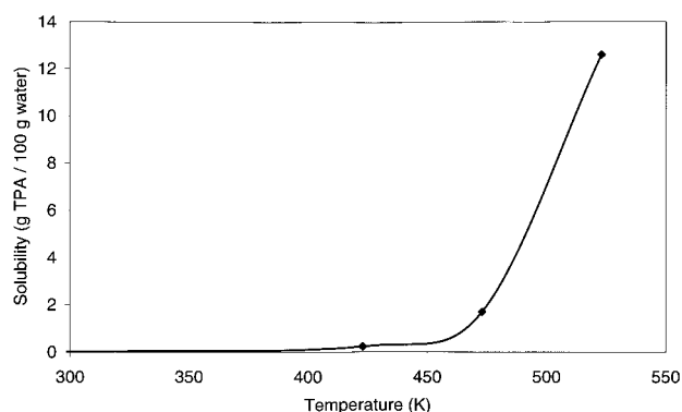
Figure 2. Variation in solubility of terephthalic acid (TPA) in liquid water with temperature.
