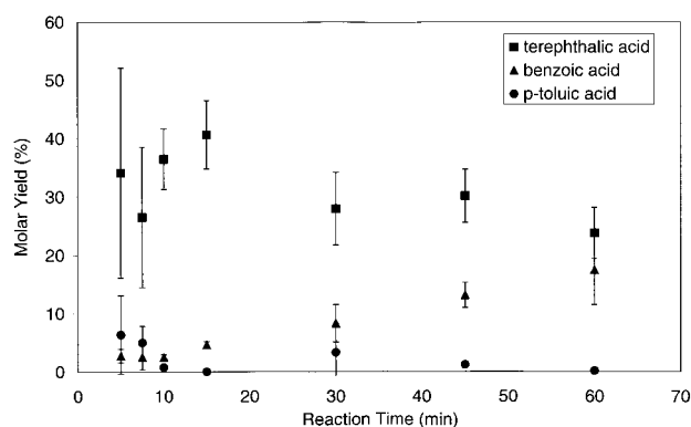
Figure 4. Temporal variation of product yields from p -xylene oxidation in SCW at 380 °C ( [p\text{-xylene}]_0 = 0.07 M, [\text{H}_2\text{O}_2]_0 = 0.91 M, [\text{MnBr}_2] = 8.4 \times 10^{-3} M, [\text{H}_2\text{O}] = 500 kg m -3 ).
