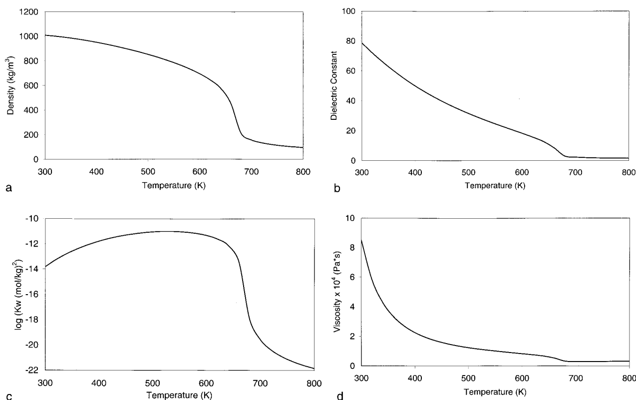
Figure 1. Variation in properties of water with temperature at 280 bar; (a) density, (b) dielectric constant, (c) ion product, (d) viscosity.
