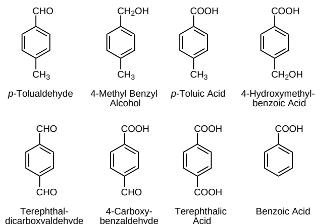
Figure 3. Reaction products identified from the partial oxidation of p -xylene in SCW.
