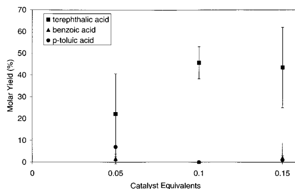
Figure 6. Product molar yields from p -xylene oxidation in SCW at 380 °C at different catalyst loadings ( [p\text{-xylene}]_0 = 0.07\text{ M} , [\text{H}_2\text{O}_2]_0 = 0.91\text{ M} , [\text{H}_2\text{O}] = 400\text{ kg m}^{-3} , t = 7.5\text{ min} ).
