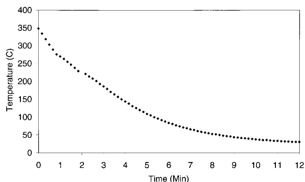
Figure 11. Temperature of a reactor loaded with water versus time as it is cooled by a fan.
